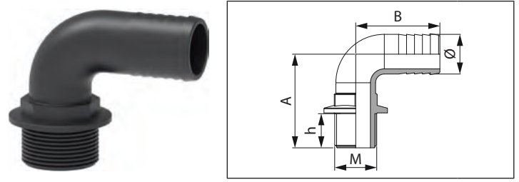
Raccordo portagomma curvo filetto maschio 90° hose fitting with male thread Racor portamanguera curvo rosca macho
