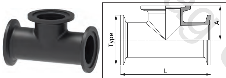
Raccordi T attacco a morsetto* 3-way Tee fitting with clamp coupling* Racores T soporte abrazadera*
