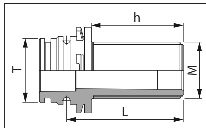
Raccordo passaparete filettato maschio attacco maschio Bulkhead male threaded with male connection Racor pasapared roscado macho con conexión macho
