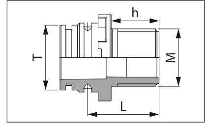
Raccordo filettato maschio attacco maschio Male threaded with male connection Racor roscado macho con conexión macho
