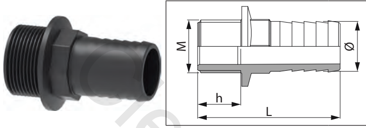
Raccordo portagomma dritto filetto maschio Straight hose fitting with male thread Racor portamanguera recto rosca macho
