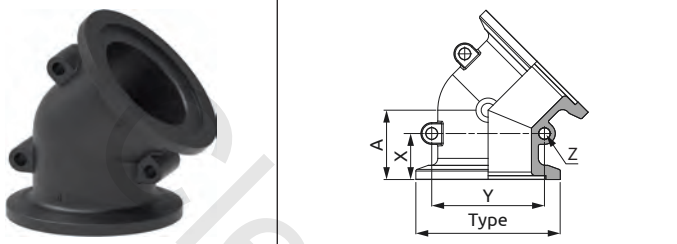
Raccordi 45° attacco a morsetto* 45° fitting with clamp coupling* Racores 45° soporte abrazadera*
